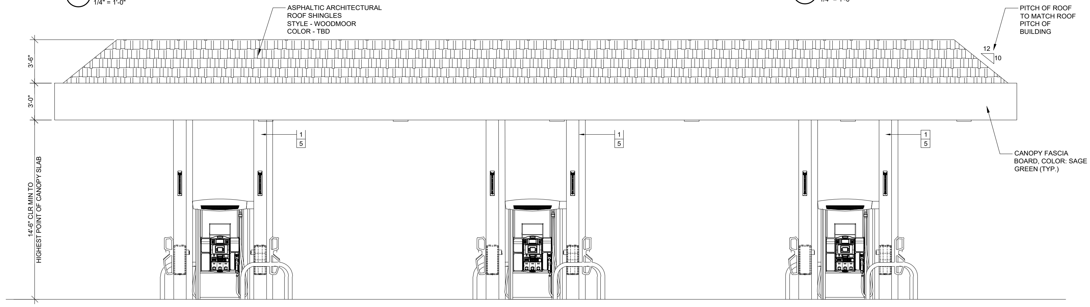
4 PROPOSED EAST & WEST CANOPY ELEVATION 1/4" = 1'-0"
