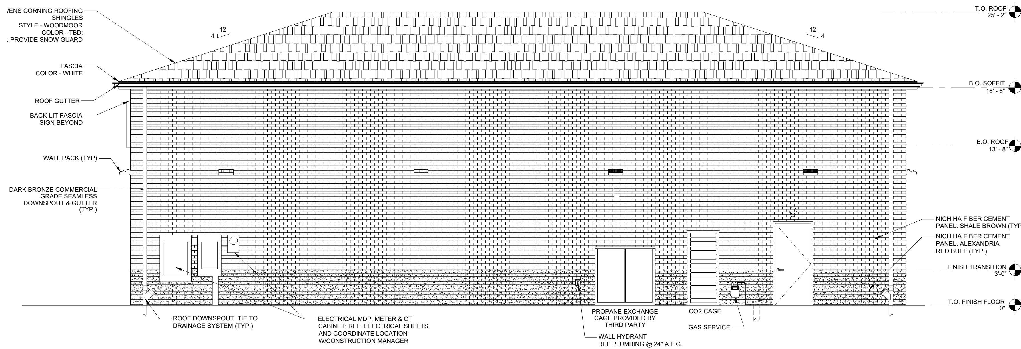
1 PROPOSED REAR ELEVATION (EAST) 1/4" = 1'-0"
