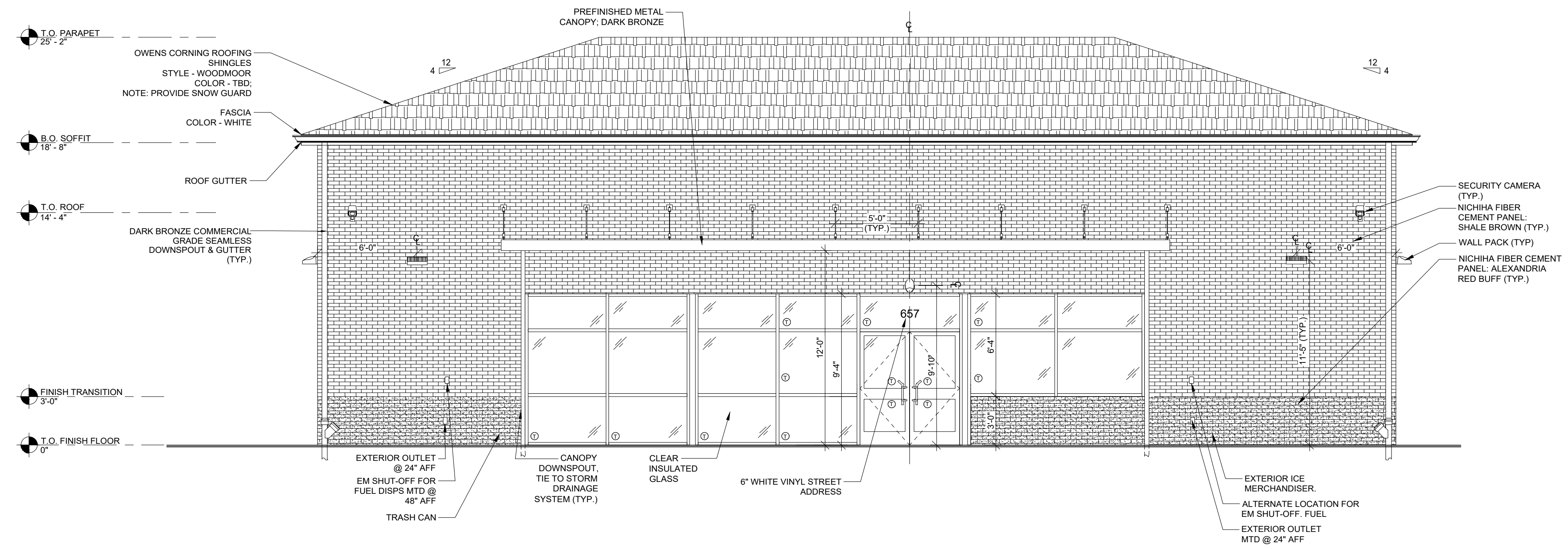
1 PROPOSED FRONT ELEVATION (SAW MILL RIVER ROAD - WEST) 1/4" = 1'-0"
