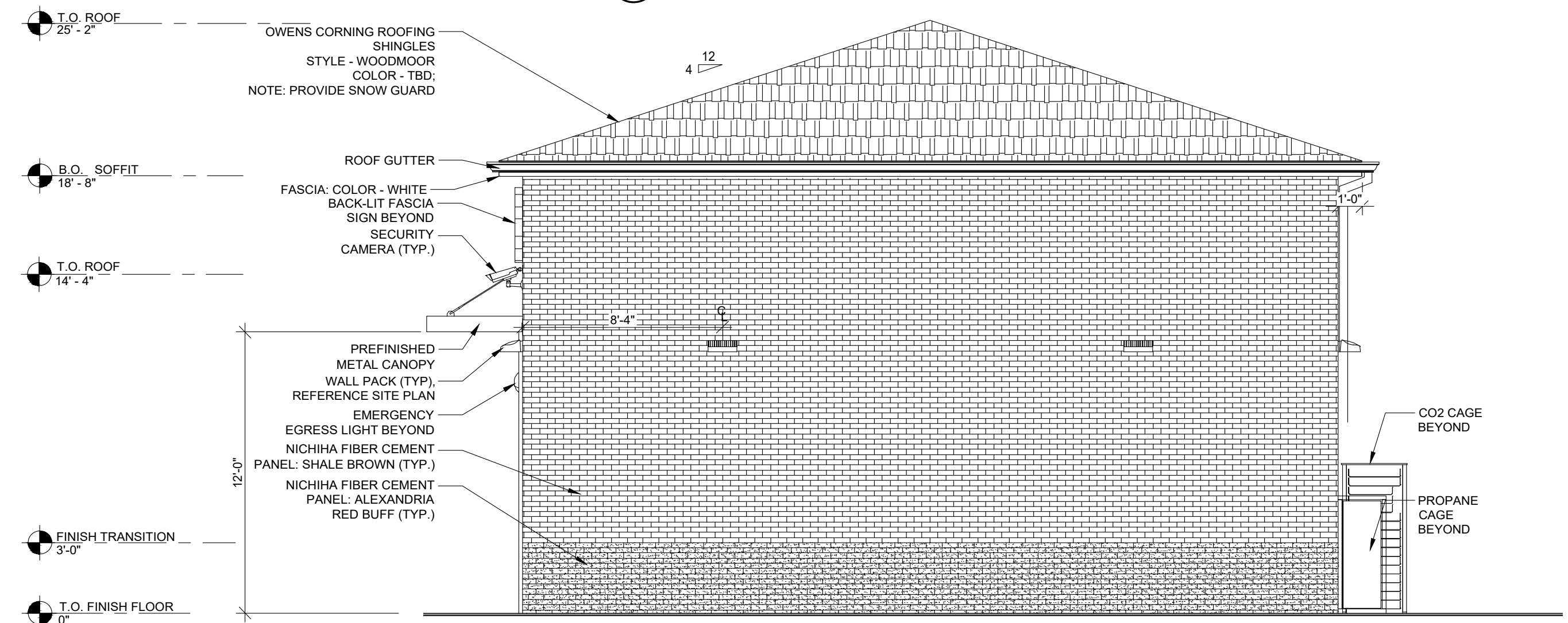
2 PROPOSED SIDE ELEVATION (RIDGE ROAD - SOUTH) 1/4" = 1'-0"
