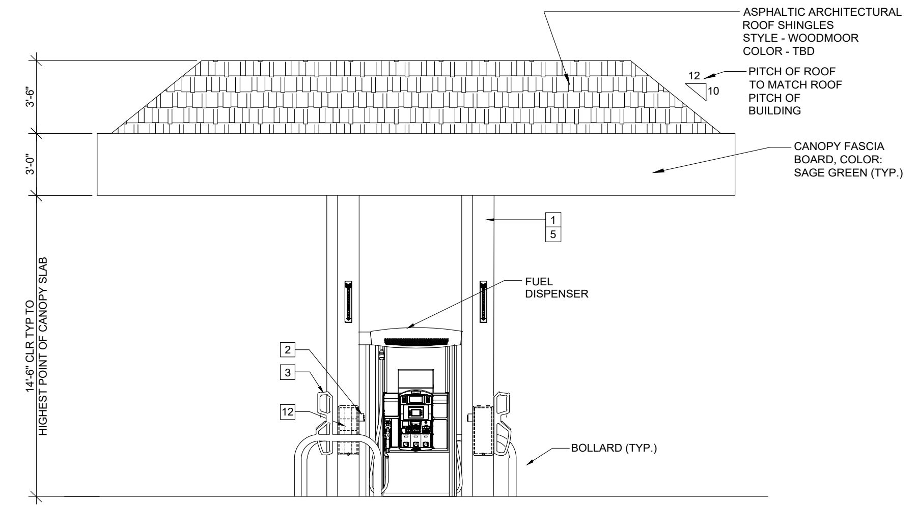
3 PROPOSED NORTH & SOUTH CANOPY ELEVATION 1/4" = 1'-0"
